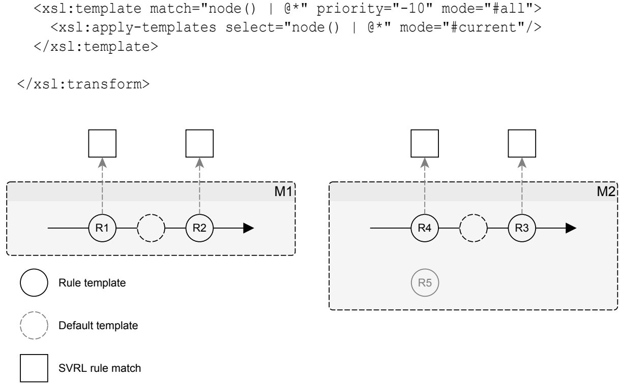
Figure 1. Processing the Rules R1–R4 in two modes
