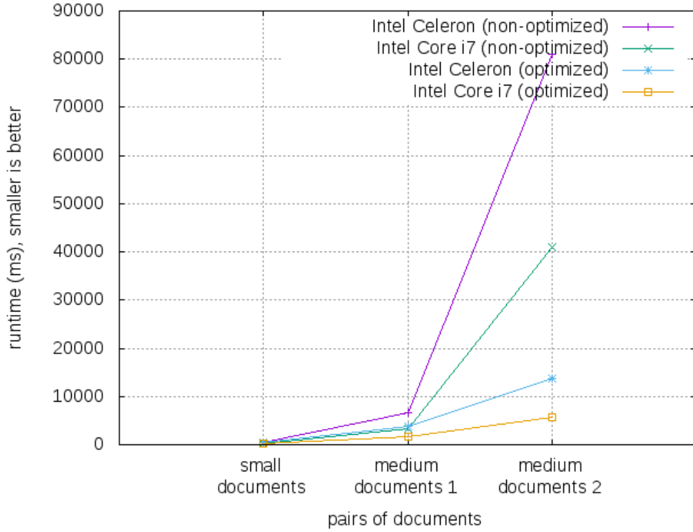
Figure 1. tagdiff runtimes
