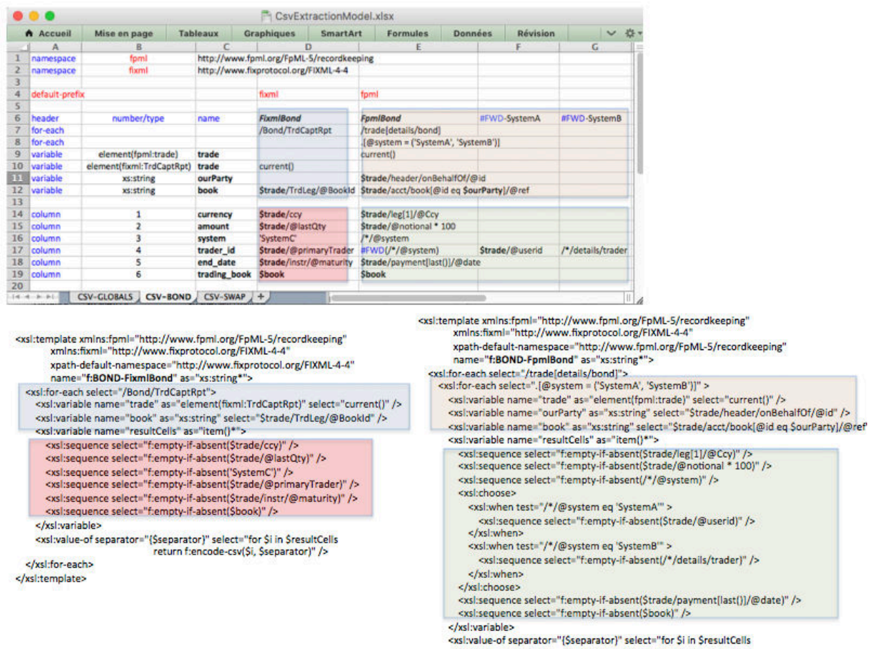
Figure 3. Association between the generated templates and the example worksheet
